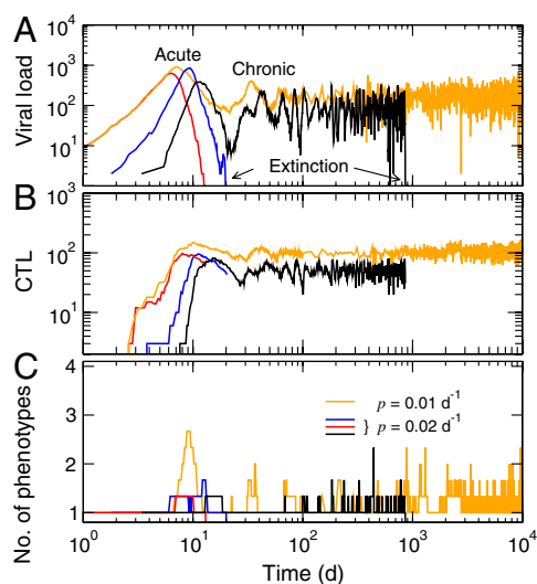
Fig. 3. Typical disease progression patterns in the extinction regime from the multi-epitope quasispecies model. (A) Viral load. (B) Total CTL levels. (C) Number of distinct phenotypes per epitope present in the population. The parameter values other than p and \mu = 1.0 \times 10^{-5} \text{ bp}^{-1} were the same as in Fig. 2. The data shown are individual trajectories.
