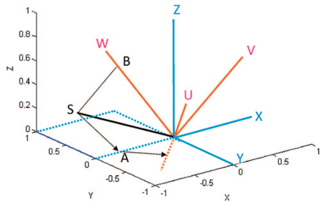
Figure 1. Order effect based on the vectors described in Appendix A. One basis is generated by the X = [1, 0, 0] , Y = [0, 1, 0] , and Z = [0, 0, 1] basis vectors. The blue X, Y, Z basis could represent three mutually exclusive and exhaustive answers to an X or Y or Z question. A second basis is generated by the U = [1/\sqrt{2}, 1/\sqrt{2}, 0] , V = [1/2, -1/2, 1/\sqrt{2}] , and W = [-1/2, 1/2, 1/\sqrt{2}] basis vectors. The orange U, V, W basis could represent three mutually exclusive and exhaustive answers to another incompatible U or V or W question. The initial state is represented by the black vector S = [-.6963, .6963, .1741] .
