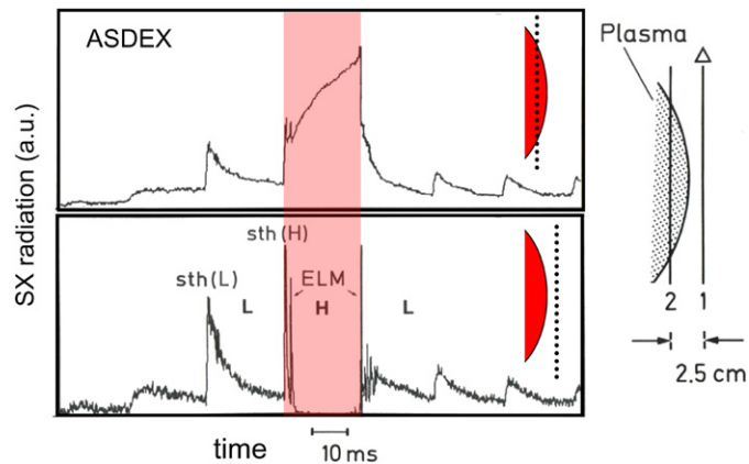
Figure 5. Transitions from OH to NBI heating. Shown are two soft-x-ray traces one inside the separatrix and the other in the SOL (see schematics at the right). The two signals are modulated by sawteeth with initially rising amplitude. The 4th sawtooth causes an H-transition developing a transport barrier at the edge. The short H-phase displays an ELM.
