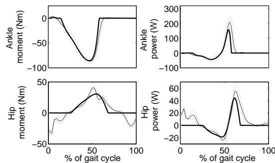
Fig. 2. Optimization Results. The sagittal plane ankle and hip moment and power are plotted for the model and biological data. The solid thin line is the mean of the human gait data ( n = 7 walking trials), and the dashed lines are one standard deviation about the mean. The solid thick line is the model or simulation curve. All curves start at heel strike (0% gait cycle) and end with the heel strike of the same leg (100% gait cycle).
