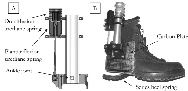
Fig. 4. Ankle and Foot Springs. In A), a section view of the ankle joint sub-assembly is shown with two urethane springs. The dorsiflexion spring is compressed from heel strike to foot flat. The plantar flexion spring is engaged as the shin rocks forward during mid-stance. In B), the ankle sub-assembly is shown attached to a modified military boot via a carbon plate for compliance for subtalar joint inversion/eversion.
