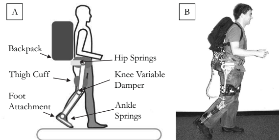
Fig. 3. Quasi-Passive Exoskeleton. In A), the main interface and joint components of the exoskeleton are shown. The exoskeleton was designed to provide a parallel load path to transfer the weight of the backpack directly to the ground. A standard military issued backpack, Alice Pack, was selected to carry the load. A carbon fiber harness connected rigidly to the backpack frame to transfer the load from the backpack to the exoskeleton. The exoskeleton interfaced to the human via shoulder straps, a waist belt, thigh cuffs, and a shoe connection. The degrees of freedom were chosen to minimize kinematic constraints experienced by the wearer and joint ranges of motion accommodated normal human walking. Further, the physical connection between the exoskeleton and the human enabled the exoskeleton to passively track the humans leg motion. In B), a participant is shown walking with the exoskeleton.
