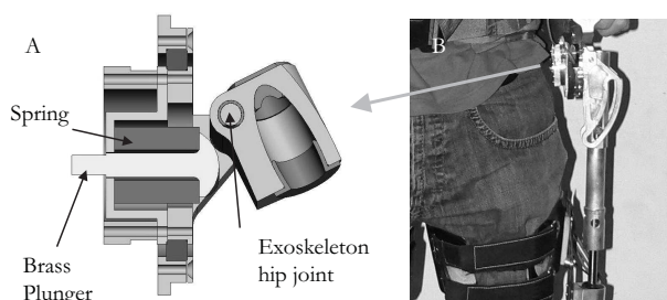
Fig. 7. Hip Abduction Spring. In A), a coronal section drawing is shown of the abduction spring sub-assembly at the hip joint. It is uni-directional so it allows the leg to freely abduct. The spring is kept in place by means of a keeper that attaches to the exoskeletal hip joint assembly. The keeper is grounded to the sagittal plane bearing so that the keeper rotates with the exoskeletal leg. A brass plunger fits through a hollow spring, allowing the spring to be compressed during hip abduction. In B), a view of the abduction spring location is shown on the exoskeletal leg.
