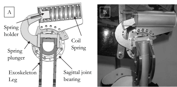
Fig. 6. Hip Flexion Spring. In A), a section view of the hip flexion spring sub-assembly is shown. The spring plunger rotates in the sagittal plane with the exoskeletal leg. The plunger engages with a spring holder and energy is stored as the spring is compressed. In B), the hip flexion spring assembly mounted on the exoskeleton is shown.
