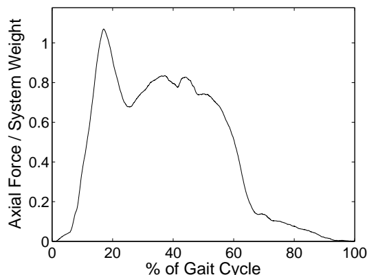
Fig. 11. Normalized Axial Force During Walking. The normalized axial force is plotted from heel strike (0% gait cycle) to heel strike of the same leg (100% gait cycle). The axial force is normalized by the exoskeleton plus payload weight equal to 467 Newtons.
