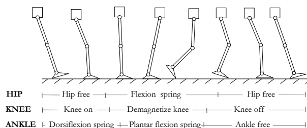
Fig. 9. Exoskeletal Joint Behavior. The sagittal plane joint behavior of the exoskeletal leg is shown from heel strike to the next heel strike of the same leg. The hip flexion spring is compressed during late-stance and this energy is released to assist the onset of the swing phase. At the knee, the damper mechanism is turned on at heel strike as the exoskeletal leg is loaded and turned off during terminal stance to allow knee flexion. The dorsiflexion spring is compressed during controlled plantar flexion and the energy is then released during the beginning of controlled dorsiflexion. The plantar flexion spring engages in controlled dorsiflexion to store energy that is later released to assist in powered plantar flexion.
