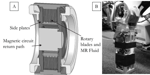
Fig. 5. Knee Variable Damper. In A), a section view of the knee sub-assembly is shown. One set of blades are grounded to the outside shell and another to the inside. When the knee rotates adjacent upper and lower blades move relative to one another, shearing the MR fluid between the blades. Using an electromagnet around the return path, a magnetic field can be modulated through the rotary blade plus MR fluid gaps, so as to change knee damping. In B), the knee variable damper is shown mounted on the exoskeleton leg.
