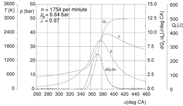
Figure 8. The results of pressure diagram analysis: rate of heat release dQ_f/d\alpha , cumulative heat released Q_f , and mean gas temperature T
