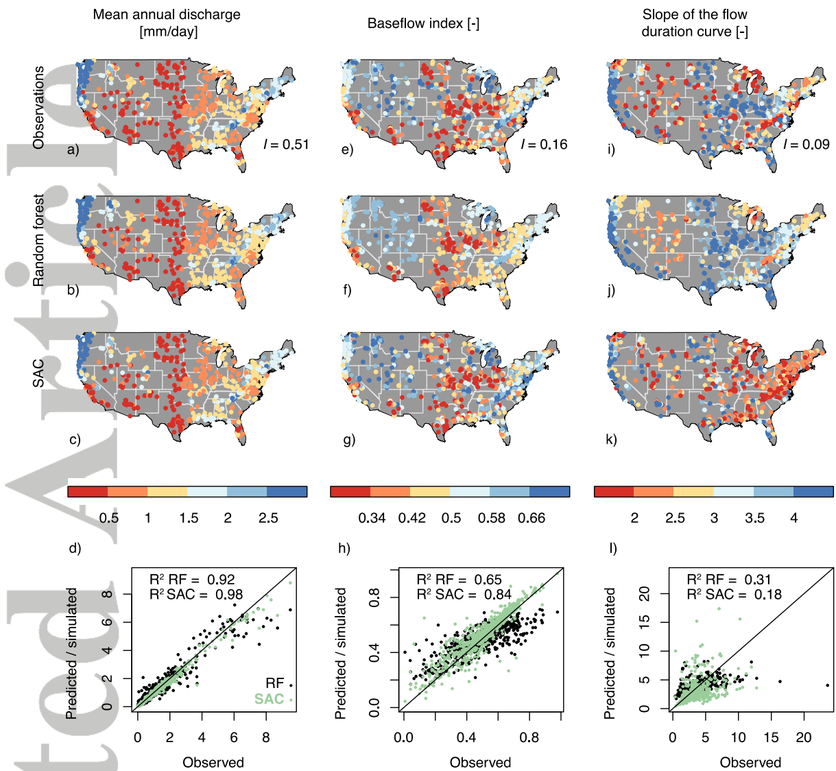
Figure 1: Comparison of the observed, predicted and simulated (first, second and third row, respectively) mean annual discharge, baseflow index and slope of the flow duration curve (first, second and third column, respectively). The spatial auto-correlation quantified using Moran's I is indicated for the maps of top row. The last row combines and compares the data from the three maps of the same column and indicates the coefficient of determination R^2 for the random forest predictions and SAC simulations computed over all the catchments.
