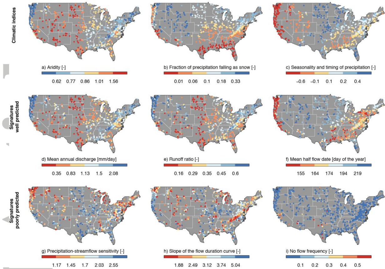
Figure 3: Comparison of the spatial patterns in climatic indices (top row), well-predicted hydrological signatures (middle row) and poorly-predicted hydrological signatures (bottom row). We used the same color scheme for all the maps to underscore similarities between them. Note that units and break values vary. The break values were chosen so that each color class encompasses about one sixth of the total number of catchments (except for the no flow frequency).
