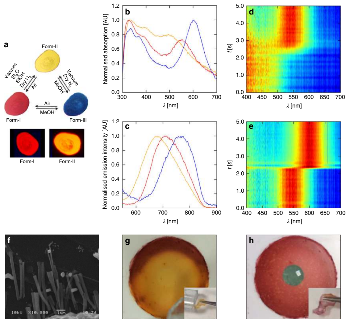
Fig. 3 Solid-state vapochromic switching in Pt-pincer complex 1 . a Images of a thin film of 1 on glass in its hydrated (Form-I), anhydrous (Form-II) and methanolic (Form-III) forms, showing the reflective (top) and emissive (bottom) colours. b, c Solid-state absorption ( b ) and emission ( c ; 500 nm excitation) spectra of the three forms. d, e Time-resolved solid-state absorption spectra of 1 during switching between the anhydrous and hydrated ( d ; Form-II \rightarrow Form-I) and the hydrated and methanolic ( e ; Form-I \rightarrow Form-III) forms. The colour scale runs from blue (minimum) to red (maximum), and each spectrum used to build the 2D plot is individually normalised to emphasise the shifts in the absorption maxima. The artefact in e during the switching is the point at which the methanol drop was applied to the film. f Scanning-electron micrograph of a similar film to those in a prepared on carbon tape, showing the microstructure. g, h Vapochromic switching in flexible polymer membranes impregnated with 1 on a support (main) and free standing (inset)
