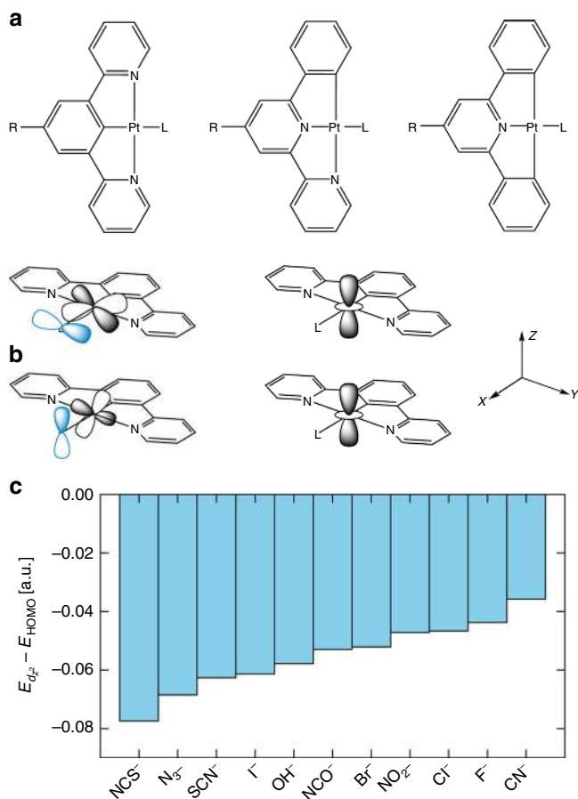
Fig. 1 Structure and electronic properties of Pt-pincer complexes. a Structure of general Pt-polypyridine pincer complexes with N ^ C ^ N ^ (left), N ^ N ^ C ^ (centre) and C ^ N ^ C ^ (right) pincer ligands. b The valence Pt d_{xy} and d_{xz} orbitals interact strongly with \pi -type molecular orbitals on the monodentate ancillary ligand (left), while the d_{z^2} orbitals of adjacent molecules can interact in the stacked geometry typically adopted in the solid state (right). c By adjusting the ancillary ligand, the energy of the d_{z^2} orbital relative to the highest-occupied molecular orbital (HOMO) can be manipulated, making the optical properties more sensitive to the solid-state stacking
