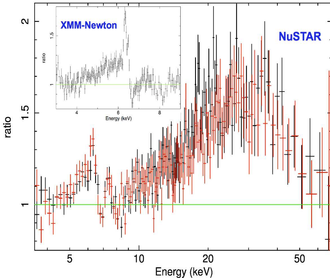
Figure 1 The broadband 3 – 79 keV X-ray spectrum of NGC 1365. An absorbed power law has been fit to the usually featureless continuum intervals 3-4 keV, 7-10 keV, and 50-80 keV. The residuals relative to this fit are shown for NuSTAR modules A and B (black and red data in main panel), and for the XMM PN (inset panel). Three prominent features are apparent: an asymmetric excess between 5 and 7 keV, a broad prominent excess between 10 and 79 keV, and a series of absorption lines between 6.7-8.3 keV. The latter are due to absorption by a highly ionized plasma 19 , which we include in all the spectral models discussed below. The two former are typical signatures of relativistically blurred emission. Quoted errors refer to a 90% confidence level.
