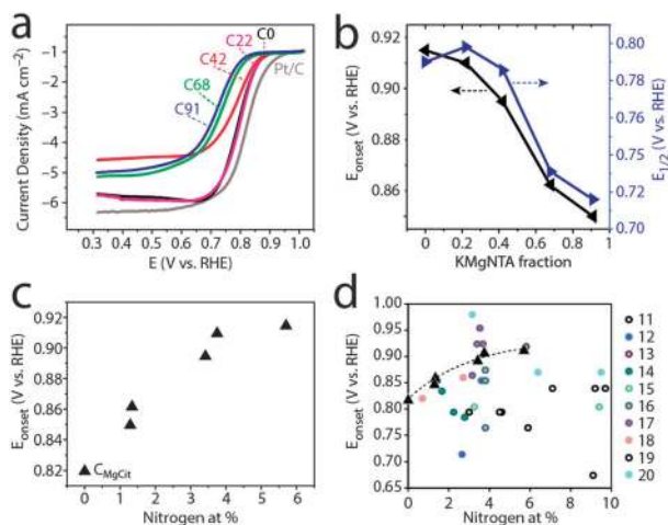
Fig. 5 Oxygen reduction activity in base (0.1 M KOH, pH 13). (a) Linear scan voltammetry, 10 \text{ mV s}^{-1} , 1600 rpm, \text{O}_2 -saturated solution. (b) Onset and half-wave potentials for ORR. (c) Onset potentials vs. total N content (at%). (d) Onset potentials from this study (triangles) plotted on literature data; 11–20 see Fig. 1 caption for details.
