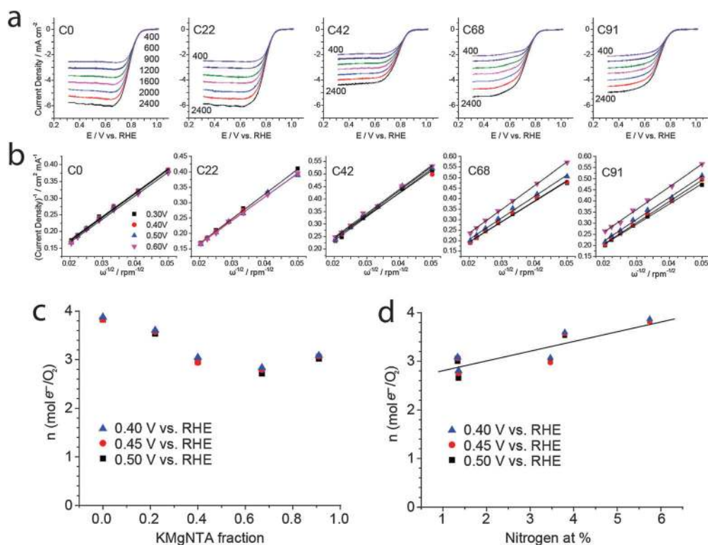
Fig. 6 Rotating disk electrode (RDE) studies of ORR electrocatalysis in 0.1 M KOH along the carbon series. (a) LSVs at different rotation speeds in rpm, 10 \text{ mV s}^{-1} . (b) Koutecký–Levich plots. Number of electrons transferred per mol \text{O}_2 along the carbon series, as calculated from the Koutecký–Levich plots, vs. (c) KMgNTA fraction and (d) nitrogen content; the straight line is a least squares fit.
