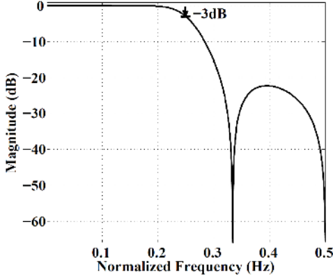
Fig. 10. Magnitude response of the HBD filter.
