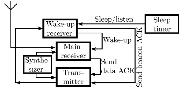
Fig. 2. Device architecture block diagram.
