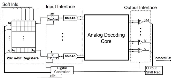
Fig. 12. Architecture of the (7,5) analog decoder with digital I/O.
