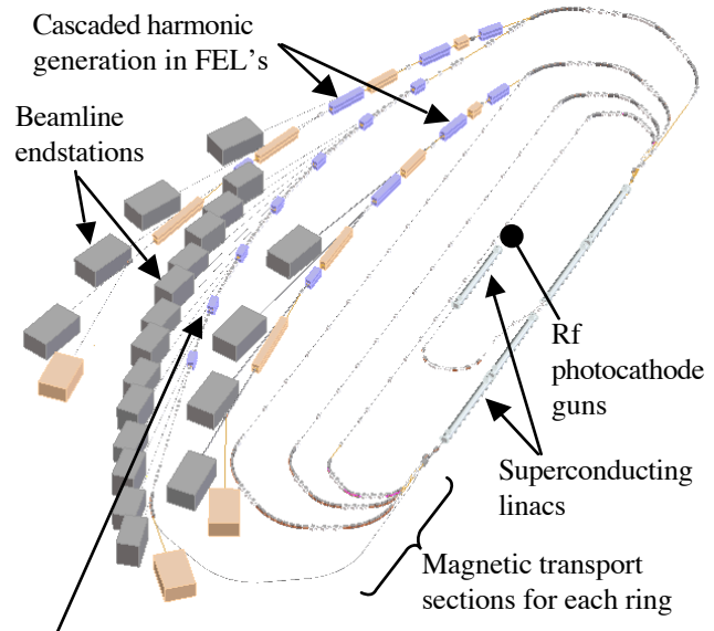
Hard x-ray production in narrow-gap short-period insertion devices
