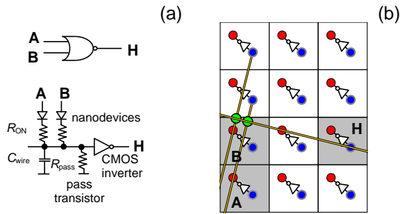
Figure 3: Fan-in-two NOR gate: (a) equivalent circuit and (b) physical implementation in CMOL. Note that in panel (b) only two (shown) nanodevices on the input nanowire of cell H are set to the ON state, while others (not shown) are set to the OFF state. For the sake of clarity panel (b) shows only the nanowires used for the gate.
