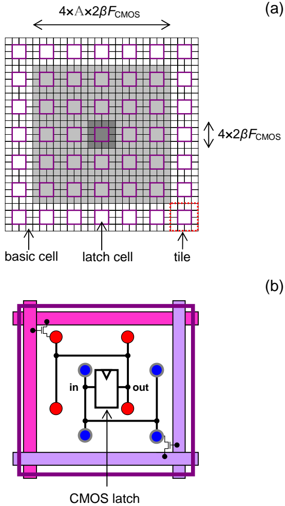
Figure 5: (a) Latched CMOL FPGA fabric and (b) latch cell structure. On panel (a), the tile connectivity domain with linear size \Delta = 5 is painted light gray. Any cell in this domain can be connected to any cell of the central tile (shown dark-gray) via a single nanowire-nanodevice-nanowire link.
