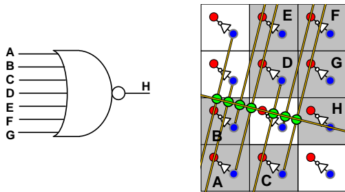
Figure 4: Example of CMOL implementation of a 7-input NOR gate. Just as in Fig. 3, only the engaged nanowires and nanodevices are shown.
