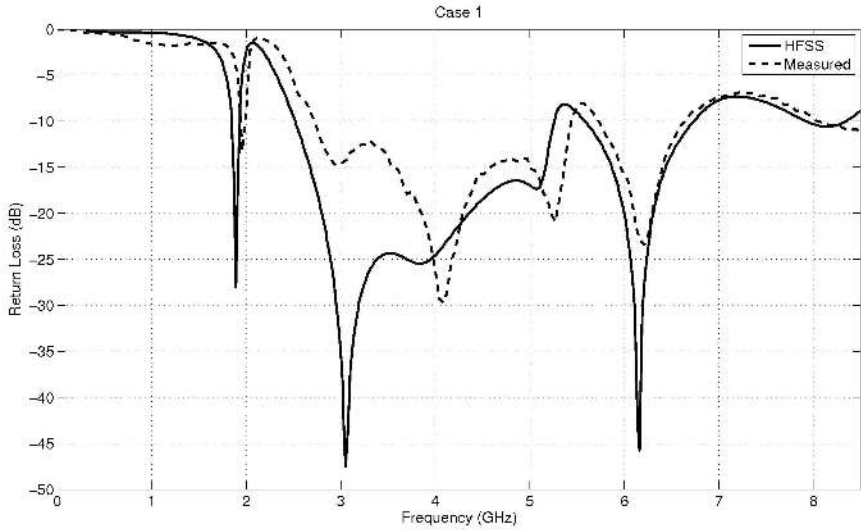
Figure 6. Simulated and measured S_{11} of the antenna for switching Case 1.
