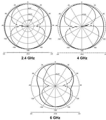
Figure 13. Radiation patterns of the antenna in X - Z plane (solid line) and Y - Z plane (dashed line) for Case 3.
