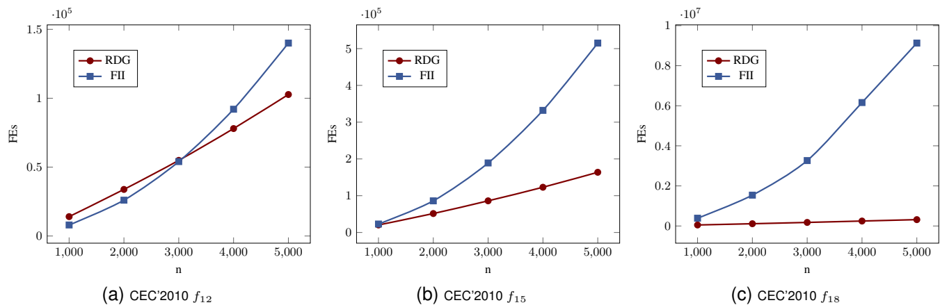
Fig. 4. The number of FEs used by RDG and FII methods when used to decompose the extended benchmark problems (CEC'2010 f_{12} , f_{15} and f_{18} ) with dimensionality equal to 1000, 2000, 3000, 4000, and 5000.
