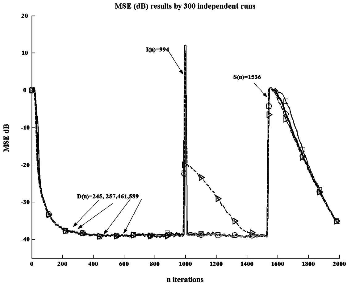
Fig. 5. MSE results for the RLM algorithm with different parameter thresholds k_\epsilon (Example 2). (1) k_\epsilon = 1.2817 (diamond); (2) k_\epsilon = 1.96 (circle); (3) k_\epsilon = 2.576 (star); (4) k_\epsilon = 3.091 (triangle).
