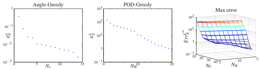
Fig. 3 Values of \epsilon_N^u and \epsilon_N^\lambda during the iterations of the greedy Algorithms 1 (left) and 2 (middle). Right: Values of Err_N^{L^\infty} with respect to N_V and N_W .
