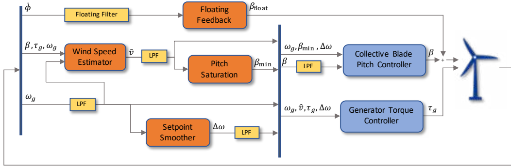
Figure 3. A block diagram showing the general controller logic in ROSCO. The generator torque and collective blade pitch controllers described in sections 3 and 4, respectively, are shown in blue. The orange squares denote the various controller modules that are described in Section 5. The yellow squares are filters. The details of the floating filter are described in Section 5.5, and the standard low-pass filter implementations are provided in Appendix A. For the feedback signals, \phi is the tower-top pitch angle, \beta is the collective blade pitch angle, \omega_g is the generator speed, and \tau_g is the generator torque. For outputs from the controller modules, \beta_{float} is the floating controller’s contribution to the blade pitch angle (see Section 5.5), \beta_{min} is the minimum blade pitch angle (see Section 5.3), \hat{v} is the estimated wind speed (see Section 5.1), and \Delta\omega is a controller reference set point shifting term from the setpoint smoother (see Section 5.2).
