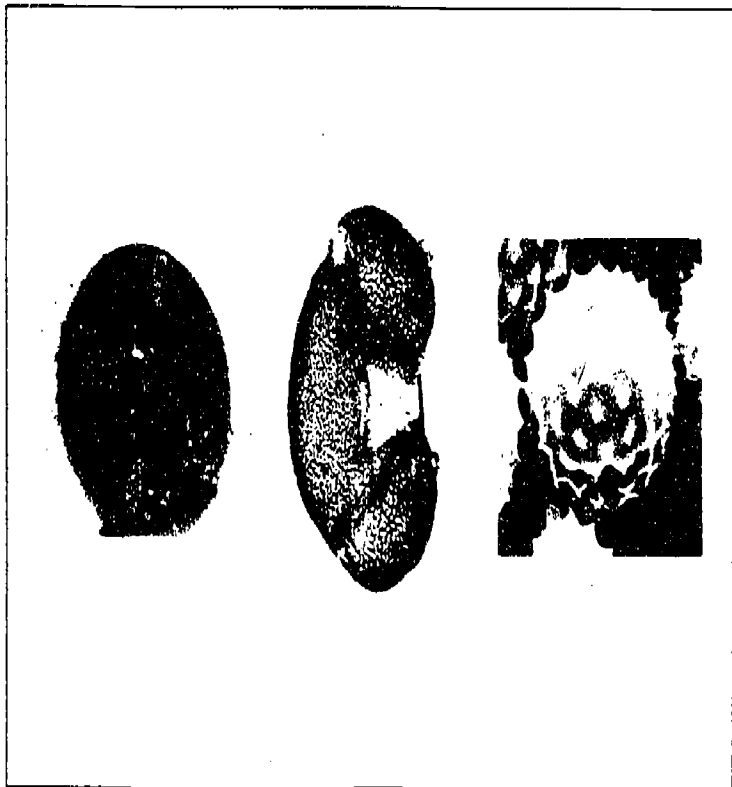
Figure 16. Microscopic views of pollen grains from glacial-age deposits provide a record of past vegetation and climate. At left is a pollen grain of Pleistocene grass (of Gramineae) x 625; middle is a grain of Pleistocene pine pollen ( Pinus sp.) x 500; and right is a modern ragweed pollen grain ( Ambrosia trifida ) x 1150 as seen through a scanning electron microscope. Photos by Richard G. Baker and Michael R. Burkart.
