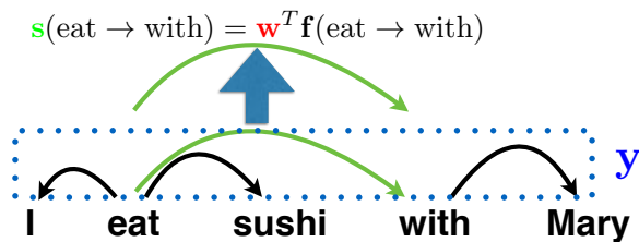
Figure 1: Three levels of representations of the parser: the parameter \mathbf{w} , the edge score \mathbf{s} , and the parse \mathbf{y} .
