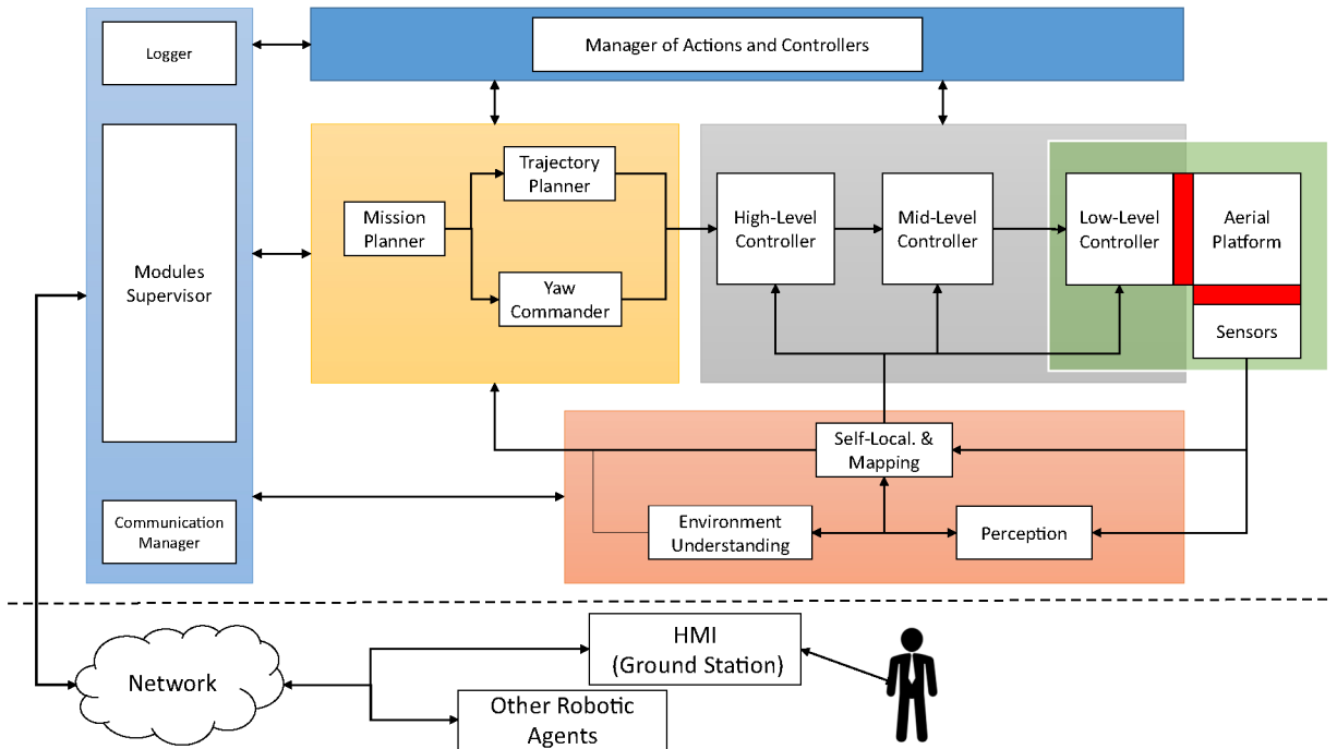
Fig. 2 Proposed Autonomous Multi-UAV System Architecture. The green block on the right symbolizes the Aerial Platform (section 2.1); the red block includes the Localization and Mapping Modules (Section 2.2); the gray block covers the Control Modules (2.3); the yellow one represents the
