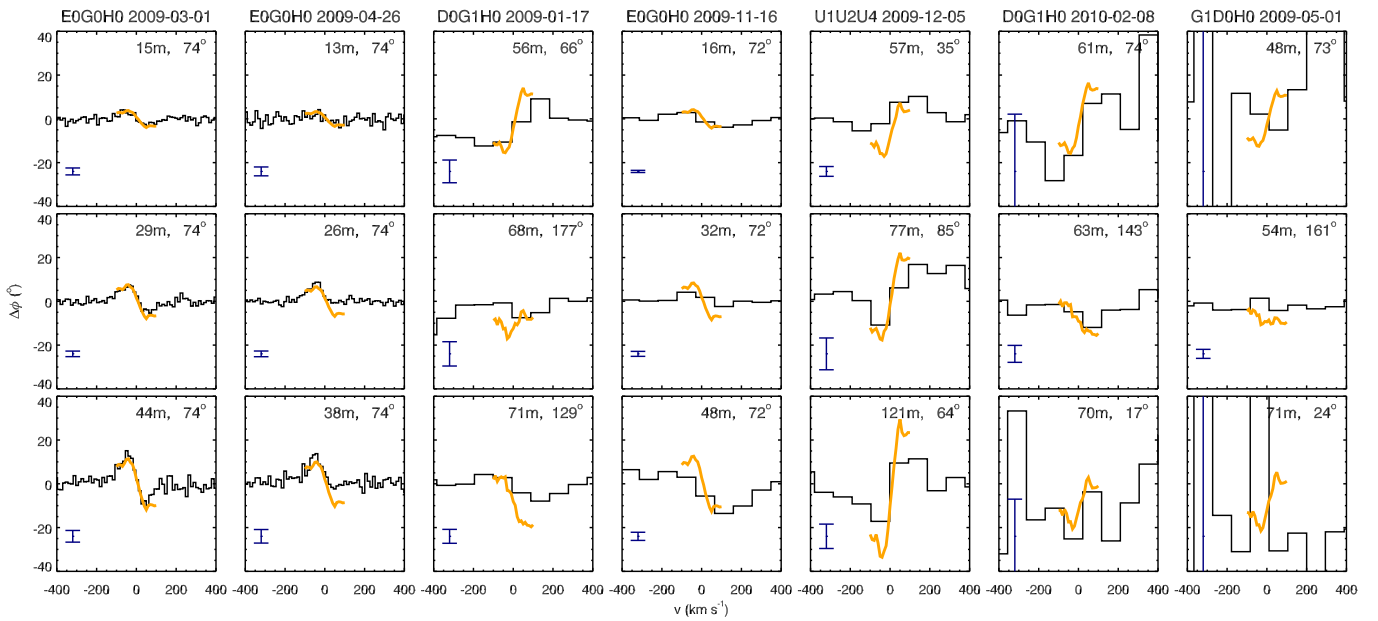
Fig. A.2. Astrometric solution, P(\lambda) , (yellow line) overlotted on the differential phase observations which were not included in the fit. The error bars correspond to the 1\sigma spread in the continuum region.
