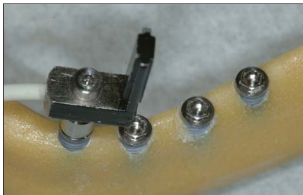
Fig 1a An Osstell transducer attached to a regular-platform (RP) Brånemark System implant parallel to the alveolar ridge of a synthetic bone model.
