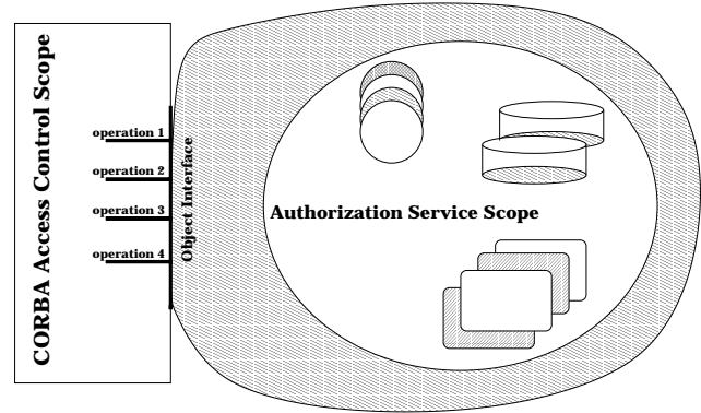
Figure 3. Scope of the authorization service
