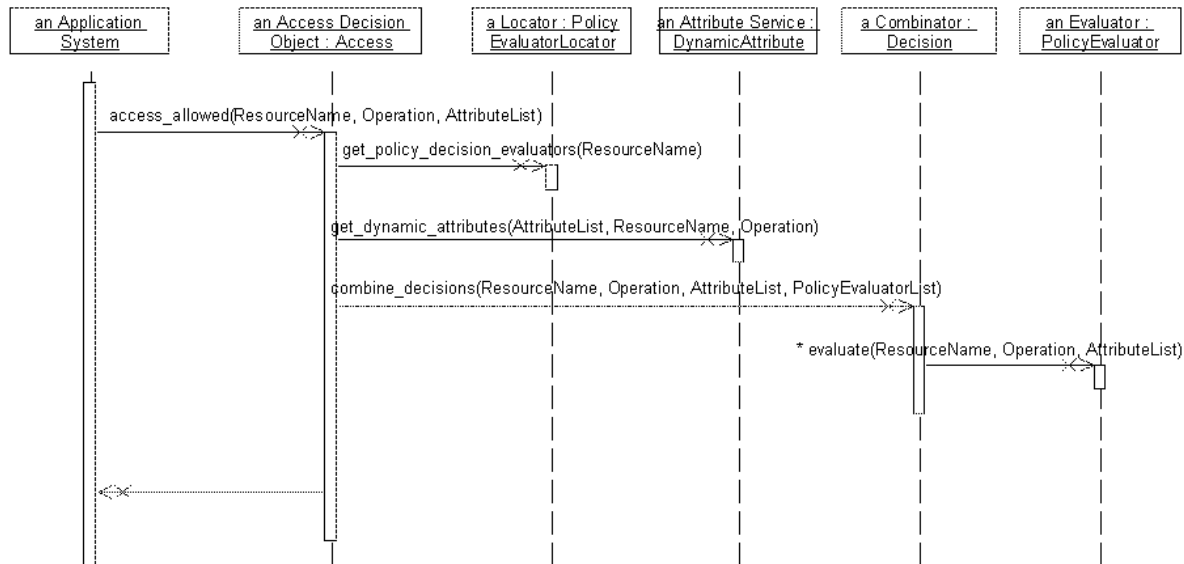
Figure 5. Interaction diagram of the authorization service components
