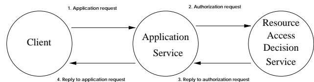
Figure 4. Interactions between client, application system, and authorization service.
