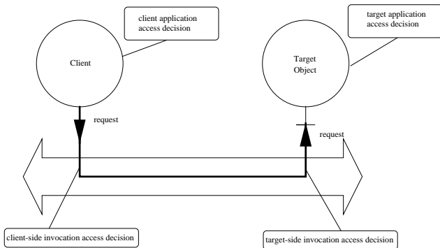
Figure 2. CORBA Security service access control model (from [3])
