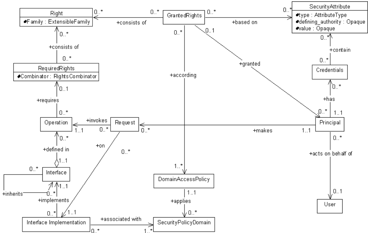
Figure 1. CORBA access control model
