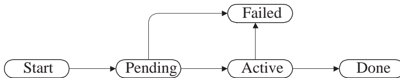
Figure 5: State transition diagram for resource allocation requests submitted to the GRAM resource management API
