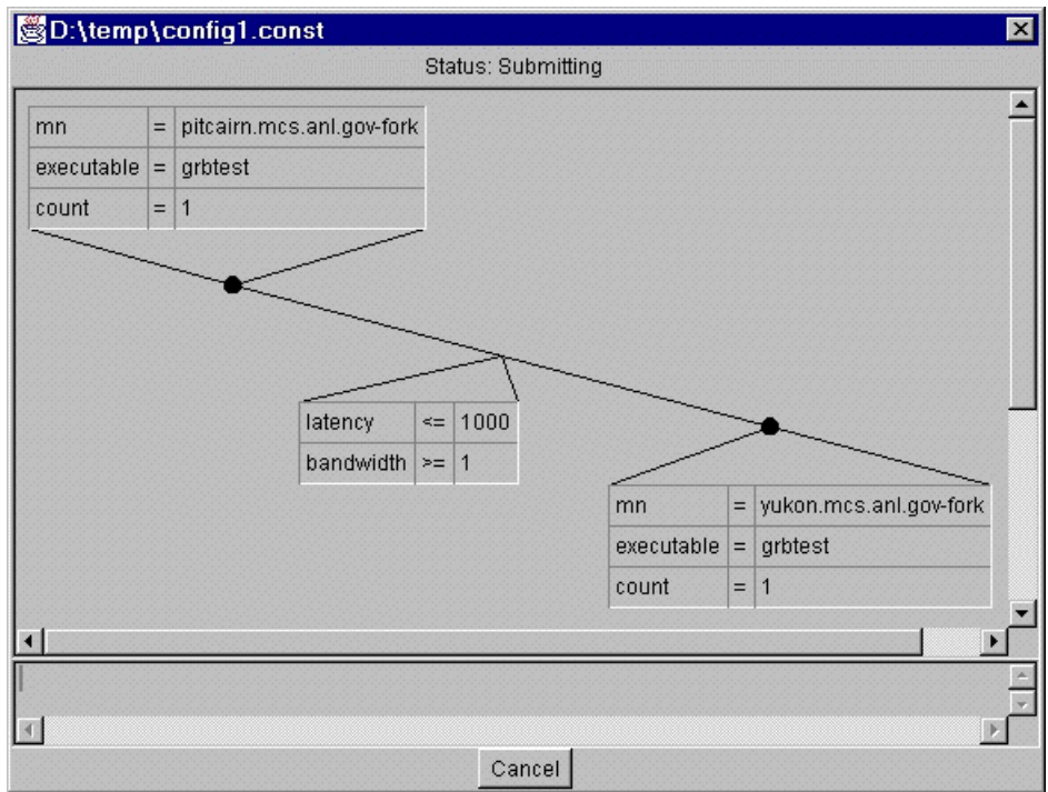
Figure 7: A screen shot of the Graphical Resource Selector. A more interesting shot will be provided in the final paper.
