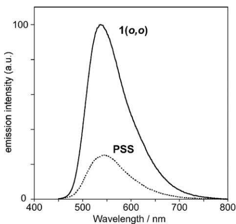
Fig. 4 Emission spectra of 1 at 298 K in cyclohexane.
