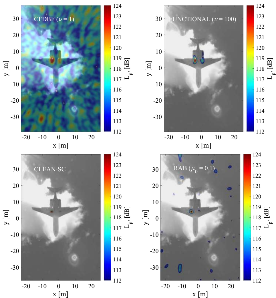
Fig. 21 Acoustic source plots for a Fokker 70 flyover at 7140 Hz. From left to right and from top to bottom: CFDBF, Functional beamforming with \nu = 100 , CLEAN-SC, and RAB with \mu_0 = 0.1 [30]
