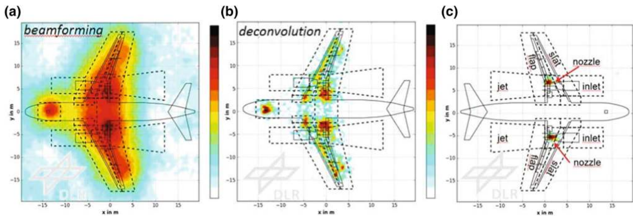
Fig. 18 a Conventional beamforming and b deconvolution source plots for a flyover measurement in landing approach for a one-third-octave-band centered at 3150 Hz. c Deconvolution source plot for a
