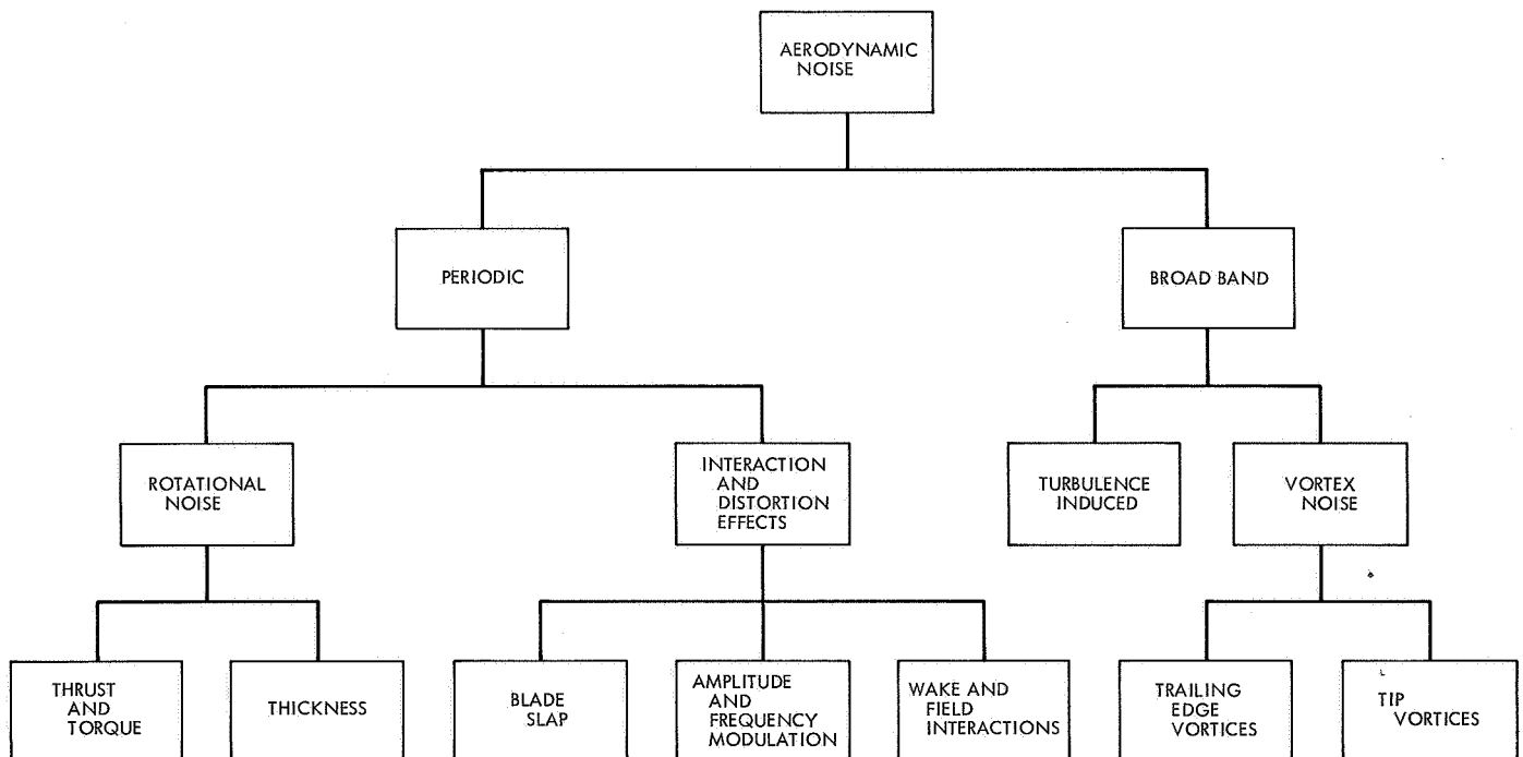
Fig. 3. Sources of aerodynamic noise
