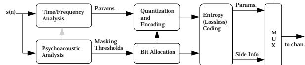
Fig. 1. Generic Perceptual Audio Encoder
