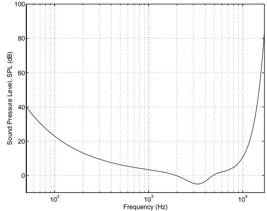
Fig. 2. The Absolute Threshold of Hearing
