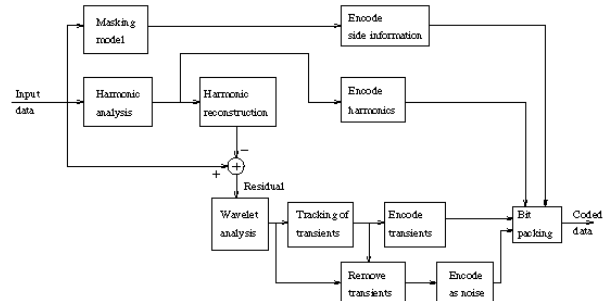
Fig. 19. Hybrid Sinusoidal/Wavelet Encoder (after [74])
