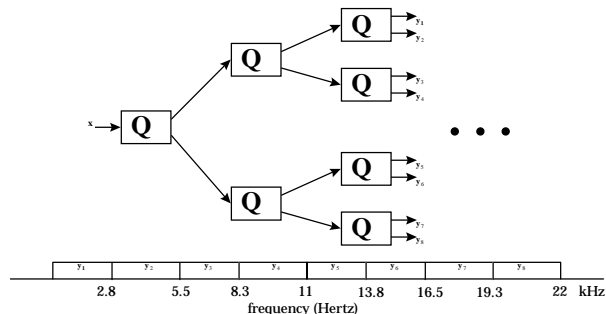
Fig. 17. Wavelet Packet Decomposition
