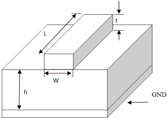
Figure 1. Basic microstrip patch antenna
