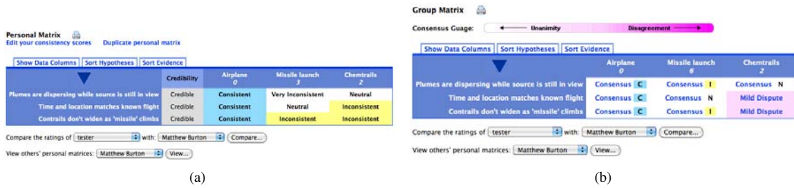
Fig. 19. In Competing Hypotheses, (a) each individual’s analysis is represented in a consistency matrix; (b) multiple analyses can be combined to create a group matrix. In the group view, darker shades of purple indicate more disagreement.
