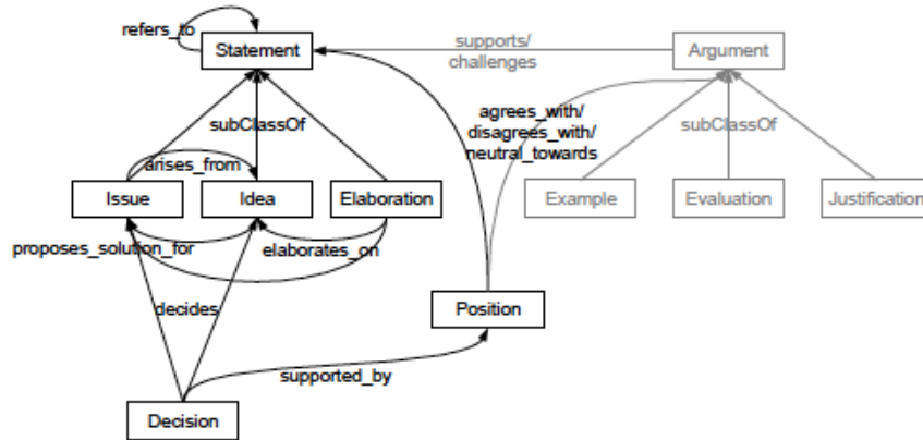
Fig. 10. An overview of the SIOC-Argumentation module from [98].
