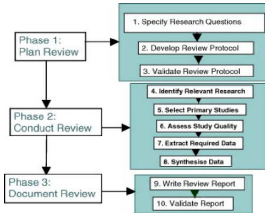
Fig. 2. SLR Methodology
