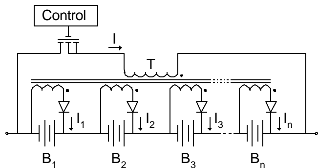
Figure 7. Shared Transformer
