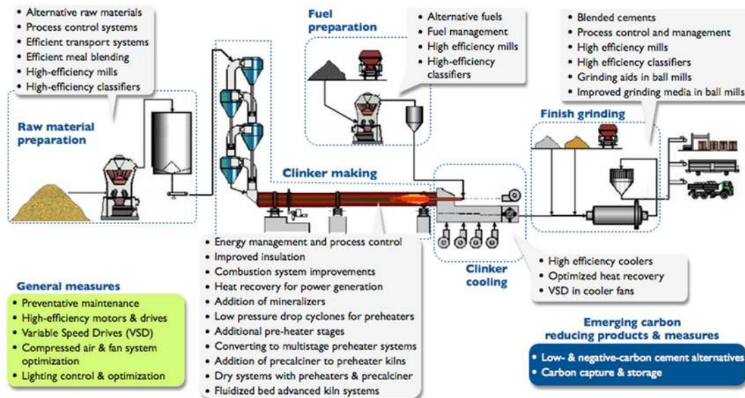
Figure 1. Energy and materials efficiency opportunities in cement sector
