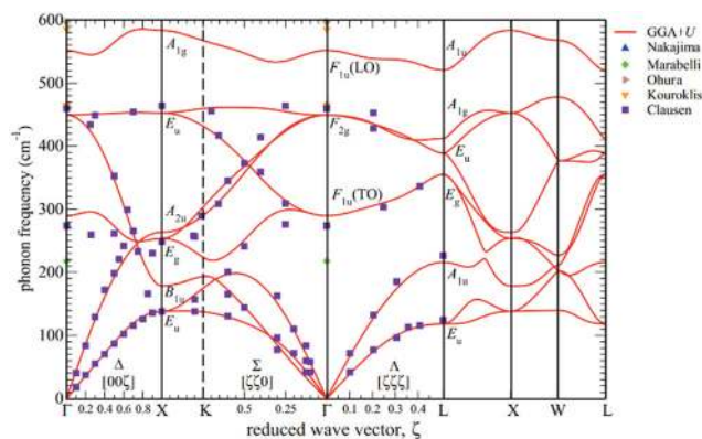
Fig. 21 Phonon dispersion plot of CeO 2 . The data lines were calculated by DFT and the data points measured by inelastic neutron scattering (purple squares), Raman scattering (blue and orange triangles), infrared spectroscopy (brown triangle), and reflectivity (green diamond). Reproduced from ref. 197, with permission from American Physical Society, copyright 2013.
