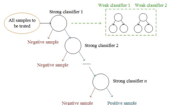
FIGURE 6. Adaboost cascading structure.
