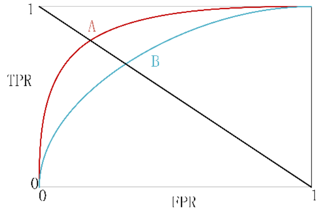
FIGURE 15. TPR – FPR curve of two different classifiers.
