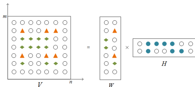
FIGURE 12. The nonnegative matrix factorization algorithm (NMF). Among them, V is the original matrix, W is the base matrix, and H is the feature matrix.
