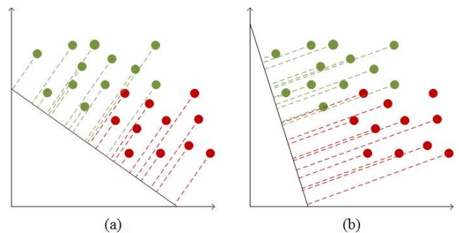
FIGURE 3. (Color online) Comparison between PCA and LDA. (a) PCA, (b) LDA.
