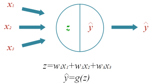
FIGURE 9. The neuron of neural network. The linear function here refers to that each neuron links the transmitted signal with weight z(x) = wx + b , while the activation function deals with the output of the neuron. The ideal activation function will map the result to '0' or '1'. Early, the Sigmoid function is more popular, and it can squeeze the output in a large range into the range of [0, 1]. Now the most commonly used function is the rectified linear unit (ReLU).
