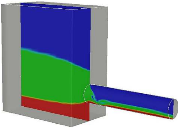
Fig. 5—Example of slag (green) and metal (red) phases during tapping from a FeMn furnace. The tap-hole diameter is 10 cm. (Color figure online).
