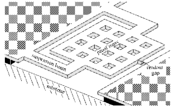
Figure 15. Schematic diagram of the tunnelling accelerometer structure. (Courtesy D F Moore et al , Department of Engineering, University of Cambridge [9].)
