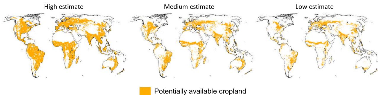
Fig. 2 Global potentially available cropland according to the high, medium, and low reproductions based on the literature review.
