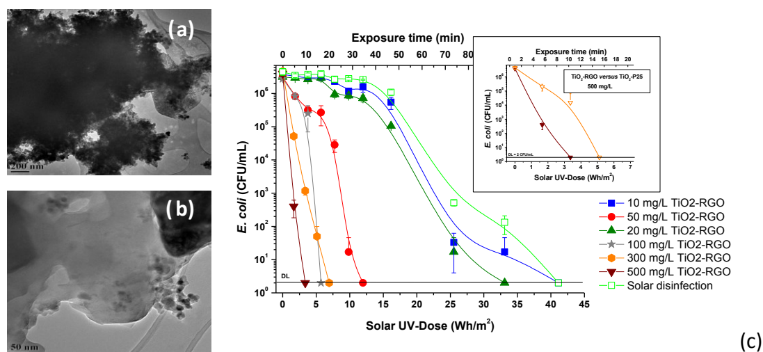
Figure 5. (a) \text{TiO}_2 -GO aggregate before photoreduction; (b) \text{TiO}_2 -RGO after UV assisted photoreduction and (c) E. coli inactivation at several \text{TiO}_2 -RGO concentrations. Figure inserts shows efficiency of \text{TiO}_2 -RGO and \text{TiO}_2 -P25 on the E. coli inactivation (reproduced from Fernández-Ibáñez, P.; Polo-López, M.I.; Malato, S.; Wadhwa, S.; Hamilton, J.W.J.; Dunlop, P.S.M.; D'Sa, R.; Magee, E.; O'Shea, K.; Dionysiou, D.D.; Byrne, J.A. Solar Photocatalytic Disinfection of Water using Titanium Dioxide Graphene Composites. Chem. Eng. J. 2015 , 261 , 36–44 [20]).
