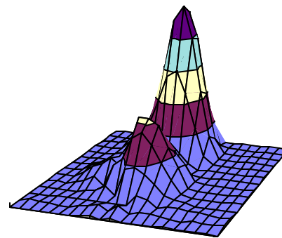
Figure 18 B - A similar HGW but with the output beam profile distorted somewhat by pushing against the side of the guide.
