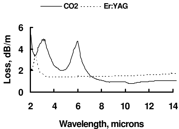
Figure 10 - Spectral response of two HGWs; one designed for low loss at the CO 2 laser wavelength of 10.6 μm and the other for low loss at the Er:YAG laser wavelength of 2.94 μm.
