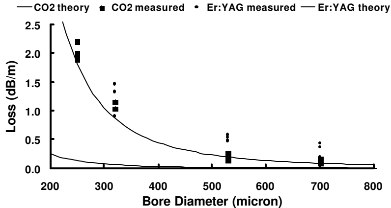
Figure 11 - Measured losses for straight HGWs using CO 2 and Er:YAG lasers. Note that the predicted losses are well below the measured ones at 2.94 μm.
