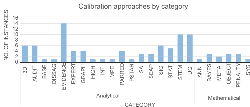
Fig. 4. Calibration approaches by category.
