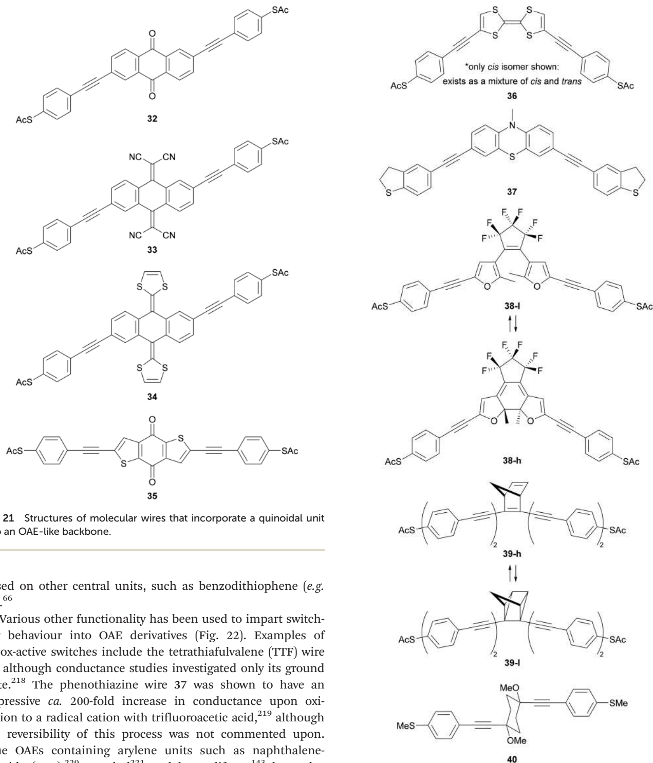
Fig. 22 OAE-like wires with switchable central units. High (h) and low (l) conductance forms of 38 and 39 are shown.
