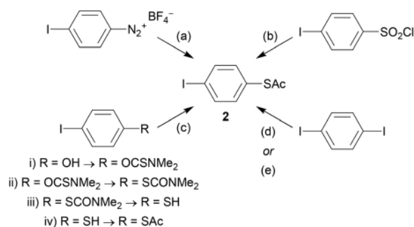
Scheme 2 Synthetic routes to 4-(acetylthio)iodobenzene ( 2 ). Reagents and conditions: (a) KSAC, DMSO, RT; (b) i. Zn, \text{Me}_2\text{SiCl}_2 , 1,2-dichloroethane, DMA, 75 °C, ii. \text{AcCl} , 50 °C; (c) i. NaH, N,N -dimethylthiocarbamoyl chloride, DMF, RT \rightarrow 80 °C, ii. 235 °C, in melt, iii. KOH, MeOH, reflux, iv. \text{AcCl} , pyridine, RT; (d) i. t -BuLi, \text{Et}_2\text{O} , -78 °C, ii. \text{S}_8 , THF, 0 °C, iii. \text{AcCl} , -78 °C; (e) KSAC, CuI, 1,10-phenanthroline, toluene, 100 °C or reflux.
