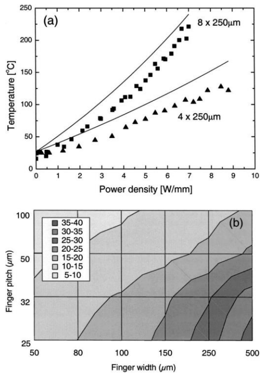
Fig. 16: (a) Temperatures measured using Raman thermography at the center of multi-finger AlGaN/GaN HEMTs with different geometries, compared to the temperature predicted by 3D finite difference modelling (solid line); (b) thermal resistance in ^{\circ}\text{C mm/W} as a function of finger width and finger spacing, predicted by thermal simulation. Reproduced from [84], with the permission of AIP Publishing.
