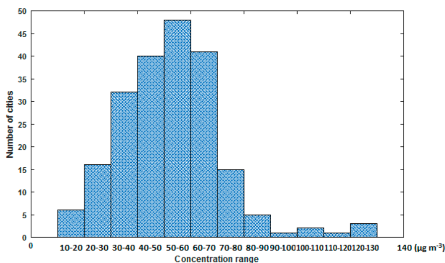
Figure 2. Histogram distribution of \text{PM}_{2.5} concentration [7].
