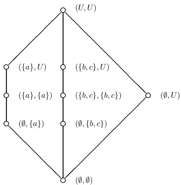
Figure 2 An example of I-rough set algebra
