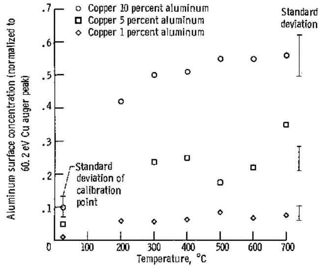
Figure 6. - Increase of aluminum surface concentration for Cu-1, 5, and 10 a/o aluminum alloys. For each point the crystal was sputtered, heated for 30 minutes, then allowed to cool to room temperature.
