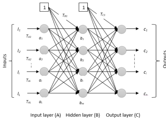
Fig. 2. Three-layered back propagation network.
