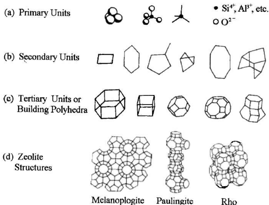
Figure 2.8. Development of a zeolite from (a) the framework PBU – the (\text{SiO}_2)^+ or (\text{AlO}_2)^5- – through (b) the SBUs and (c) CBUs to (d) a zeolite structure
