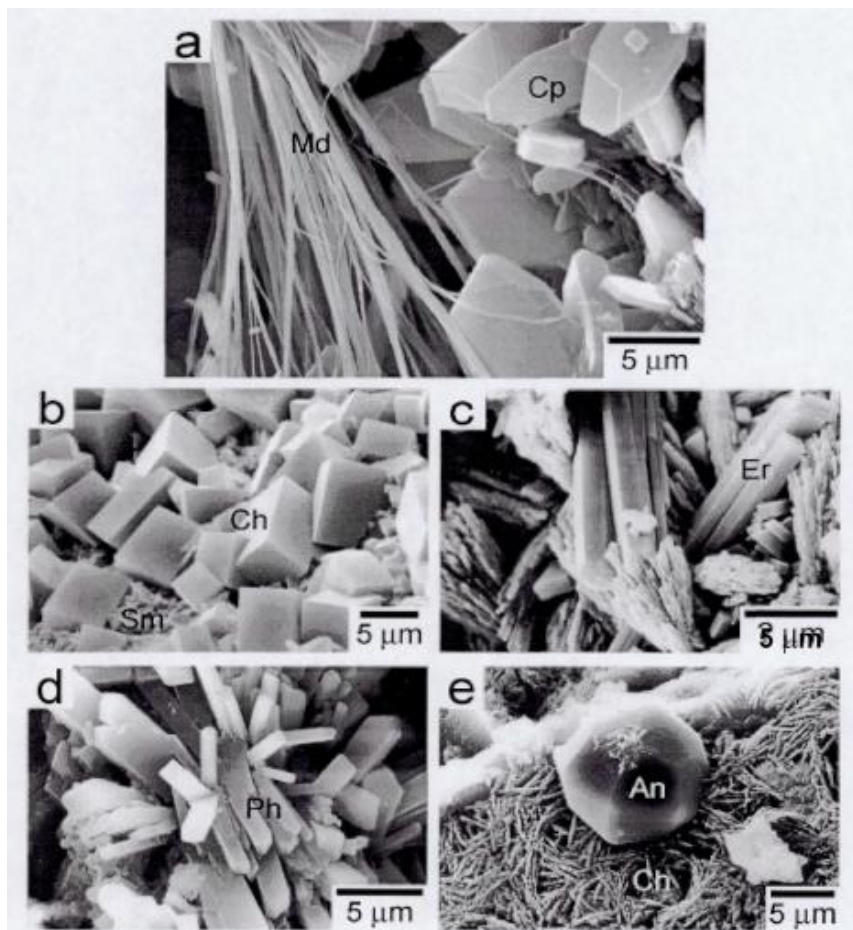
Figure 2.10. Scanning electron micrographs of common natural zeolites. a) Clinoptilolite (Cp) and modernite (Md); b) Chabazite (Ch) and smectite (Sm); c) Erionite; d) Pihstlistine and e) Analcime (An) and Chabazite (Ch) [40]
