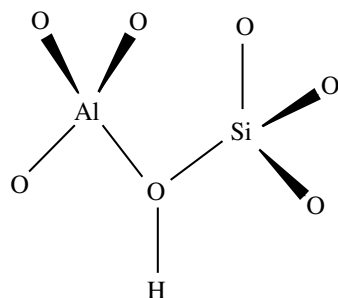
Figure 1.2. Tetrahedral arrangement of the Si-O and Al-O bonds forming a unit block of a zeolite
