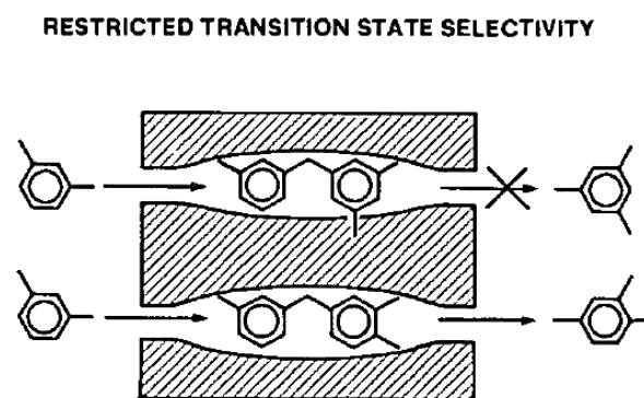
Figure 3.9. A schematic of an example of restricted transition-state selectivity through the microporous framework of a zeolite catalyst
