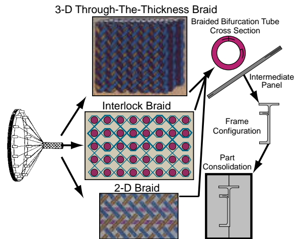
Fig. 5. Fabrication process for braided fuselage frames.
