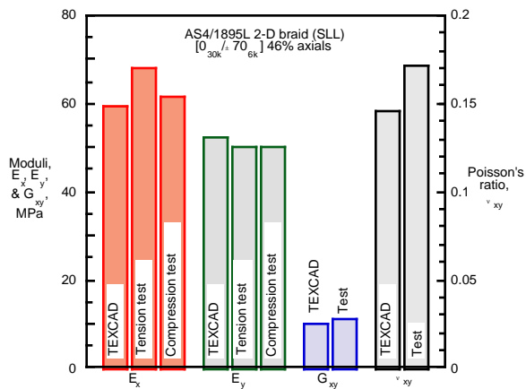
Fig. 29. Moduli by TEXCAD.
