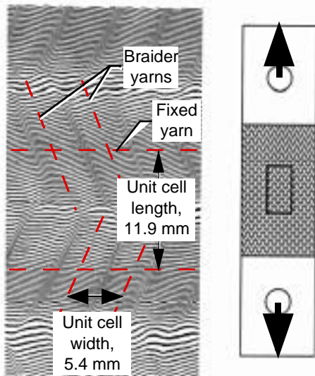
Fig. 14. Vertical displacement field in triaxial braid by Moiré.
