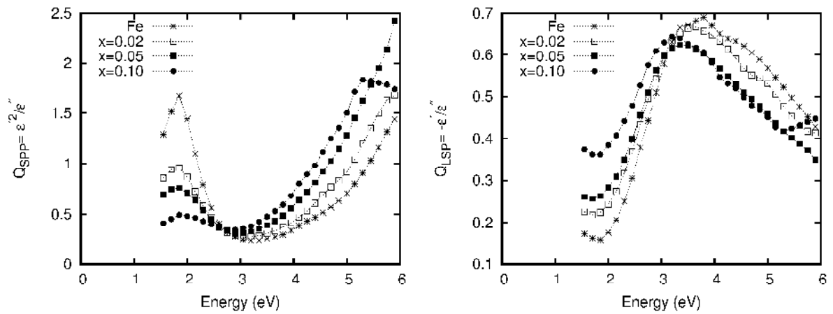
Figure 4. Quality factors for surface plasmons in the structure \text{Fe}_{1-x}\text{Si}_x
